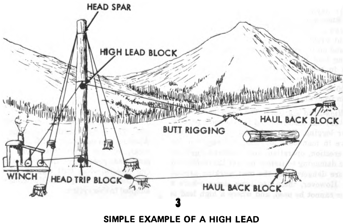
Figure 7-11. The high-lead system and its use.
